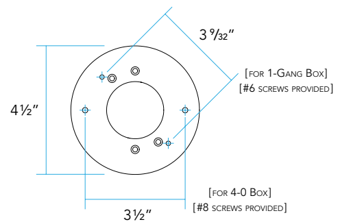
OPTIONAL ADJUSTABLE MOUNTING BRACKET
