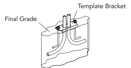
J-Bolt Anchor Assembly
