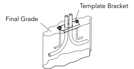
J-Bolt Anchor Assembly
