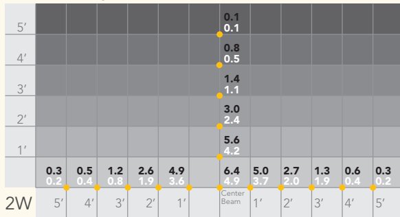
5105 2W Integrated LED
