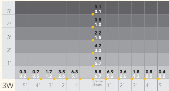
5105 3W Integrated LED
