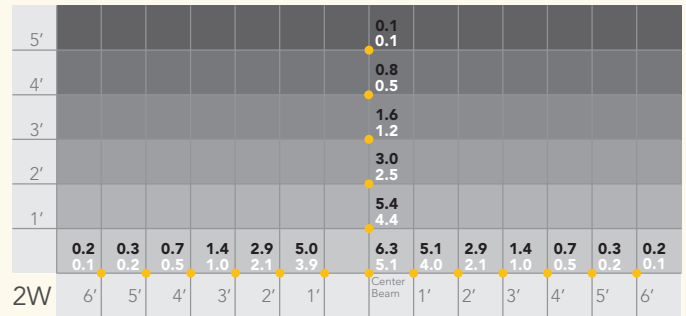
5106 2W Integrated LED
