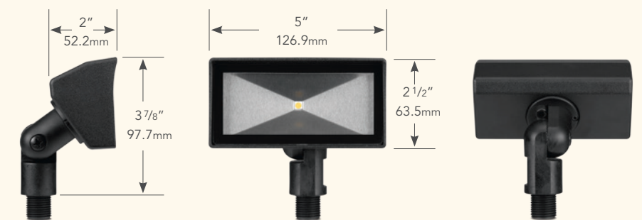
5106 front view showing single LED chip/emitter
