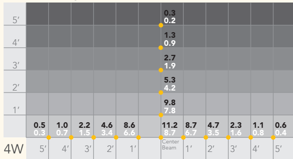
5105 4W Integrated LED
